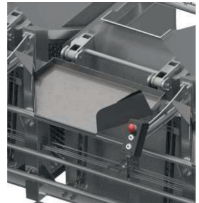
Version with buffer chute
